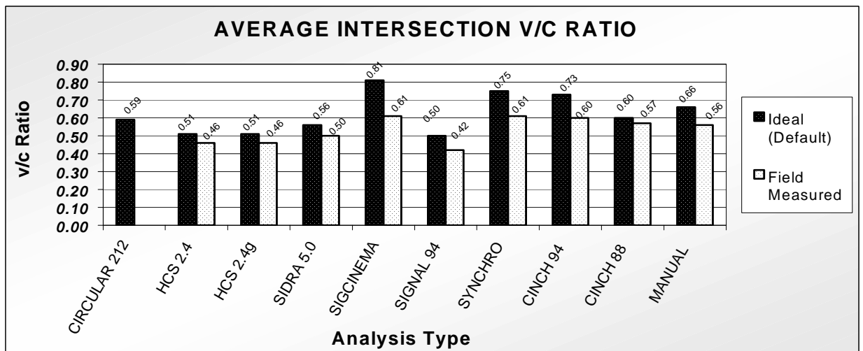
Figure 16 - Volume-to-Capacity Ratio
